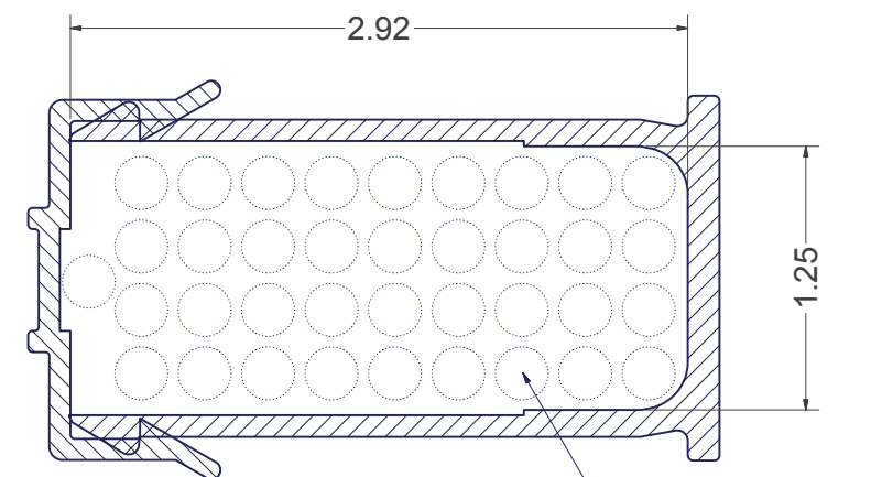
SECTION A-A SCALE 2 37X Ø.25 CABLE 50% FILL SHOWN
