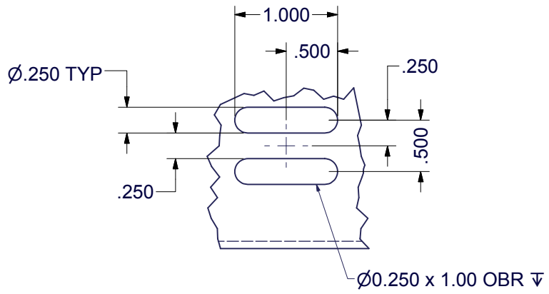
DETAIL A TYP - (28) PLC'S
