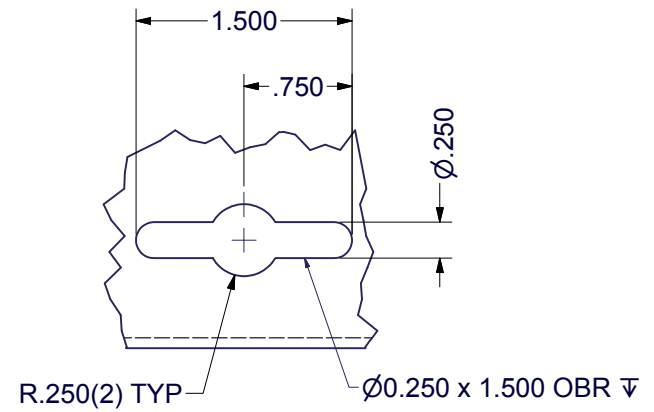
DETAIL B TYP - (4) PLC'S
