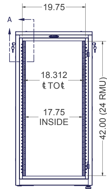
FRONT VIEW w/ DOORS REMOVED
