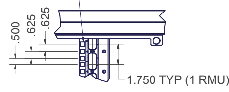
DETAIL C
