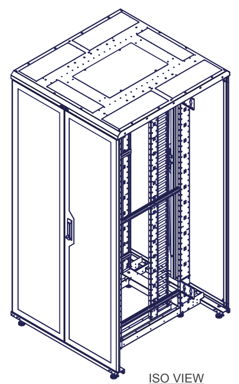
ISO VIEW
