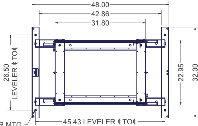
SECTION B-B DOORS REMOVED
