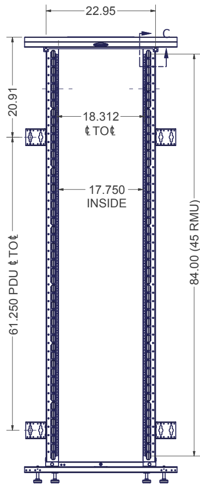
FRONT VIEW DOORS REMOVED
