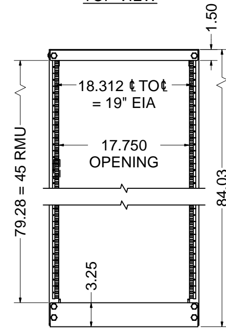
TOE IN MOUNTING TOP VIEW
