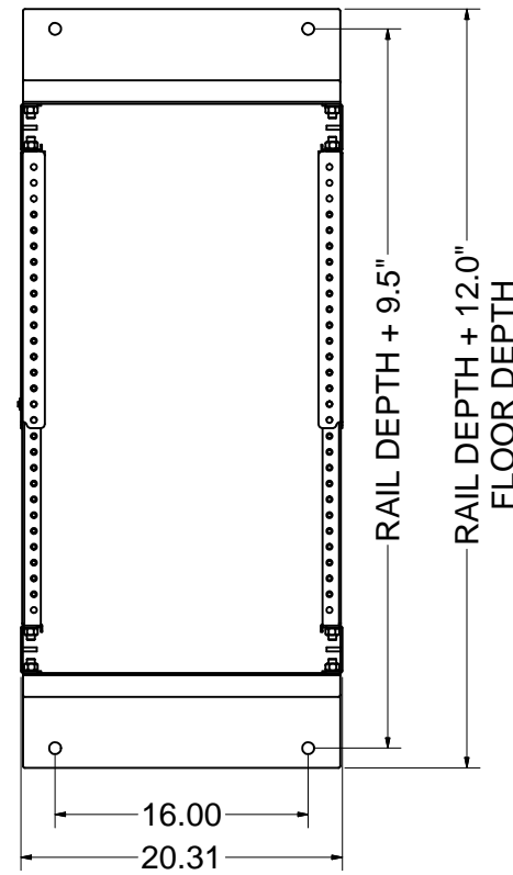
TOE OUT MOUNTING TOP VIEW
