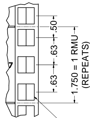
DETAIL E
