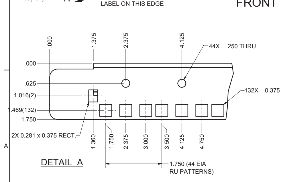
FRONT FLANGE VIEW
