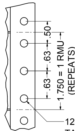
DETAIL B
