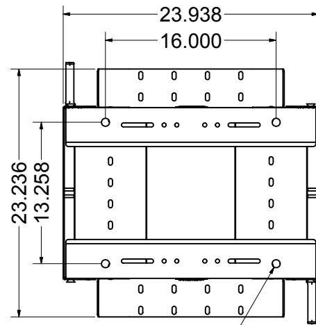
Ø.750 FLOOR MOUNTING HOLES VIEW A-A
