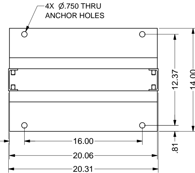
VIEW A-A SCALE .25
